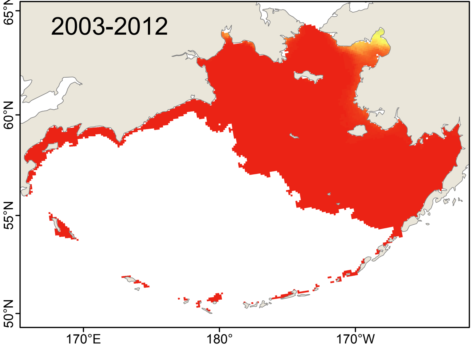
(c) Model: MIROC3.2
